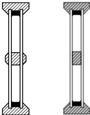
Figure J.2 — Single cross bar in the IGU with or without attached bars
